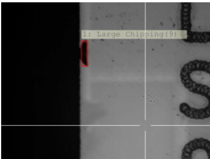
Example: Chipping examination with infrared camera.
